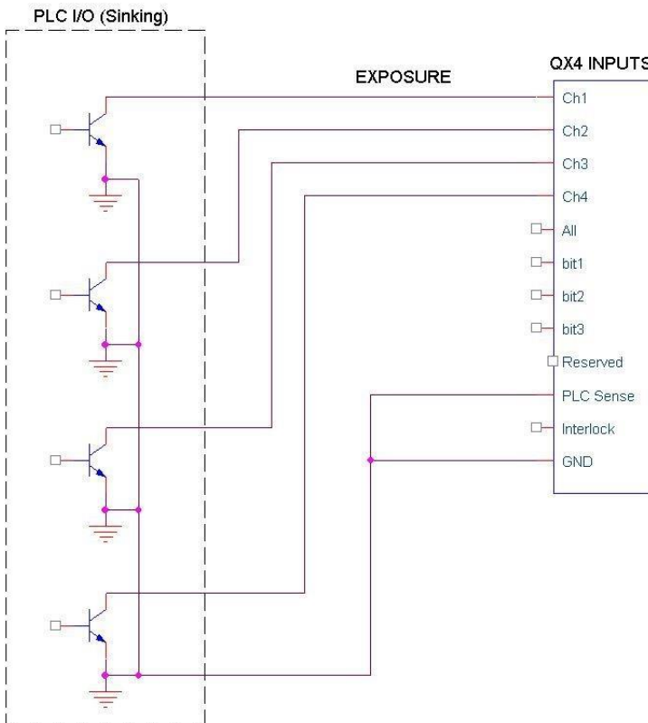
Figure 33. Connection Diagram
