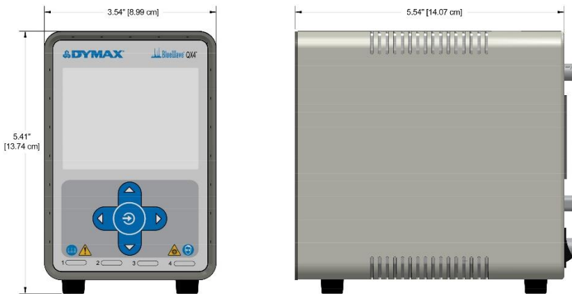
Figure 45. Dimensions - Controller
