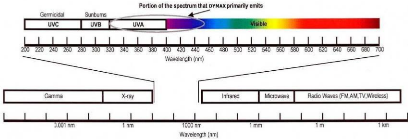
Figure 1. UV Spectrum
