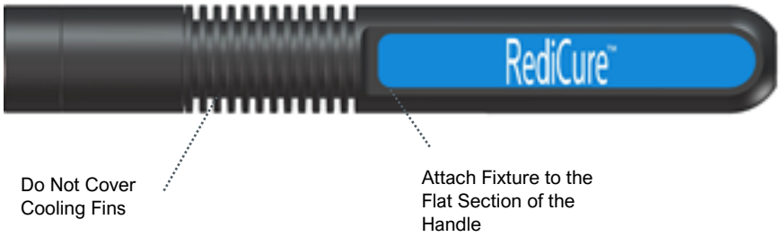
Figure 8. Fixturing Recommendations
